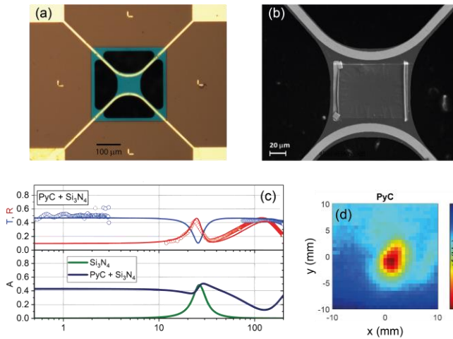
Fig. 1. (a): Microscope image of a typical TMB. (b): SEM of the PyC absorber integrated in the TMB. (c): Transmission and reflection spectra of a PyC film on Si 3 N 4 . Bottom panel shows estimated absorption obtained adding a 18 nm PyC film on the bare silicon nitride. (d): Beam profiling of the 140 GHz source using a PyC-TMB.
