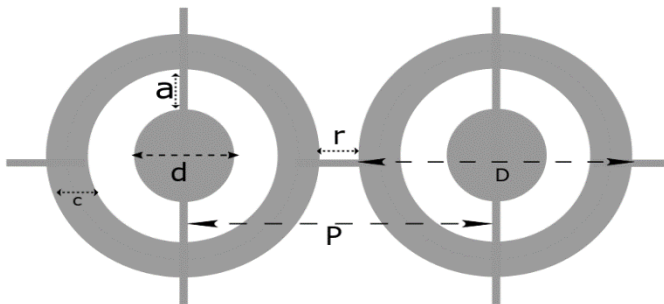
Figure 1: 2D view of metasurface of free-standing Si membrane with dimensions. a is the distance between meta-atom and unit structure, d is diameter of the meta-atom, c is the width of big ring, D is diameter of unit cell, p is the period between the unit cell, r is inter-unit cell distance.
