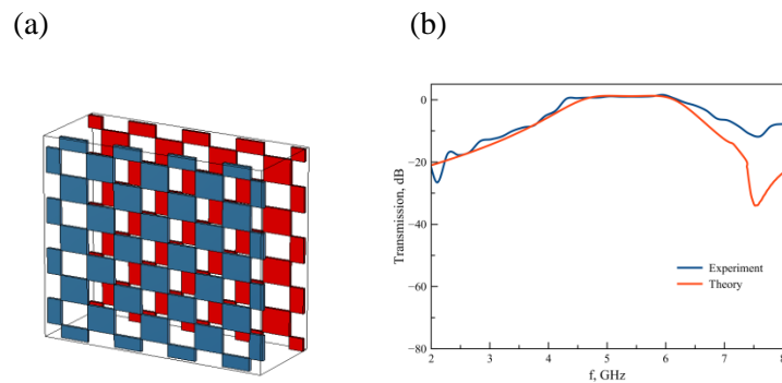
Fig. 1: Illustration of Babinet metamaterial (a) and its simulated and measured transmission characteristics (b).
